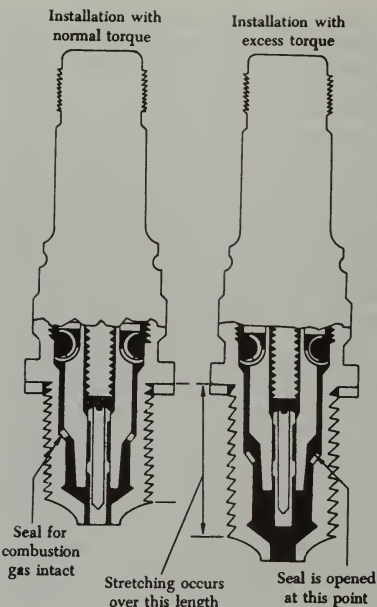
FIGURE 4-59. Effect of excessive torque in installing a spark plug.
